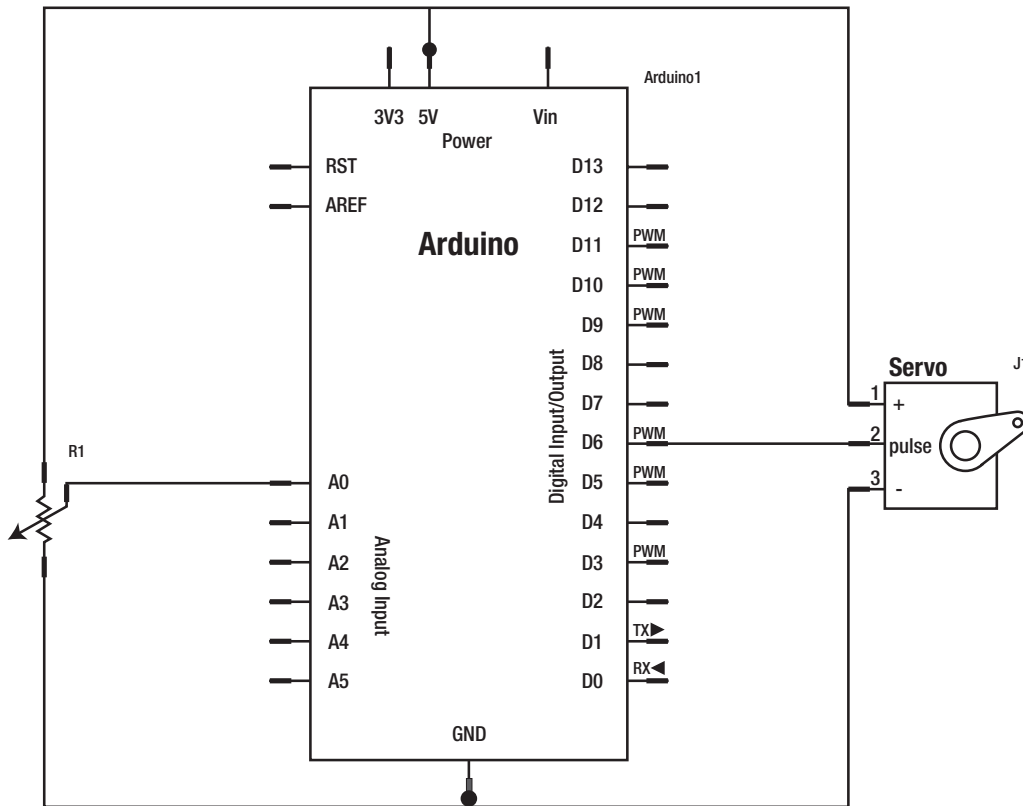
Figure 12-18. Turntable circuit
