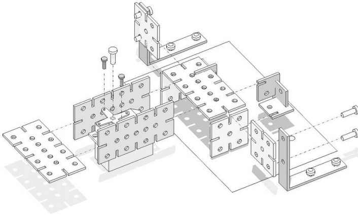
Figure 8-11. Base assembly
