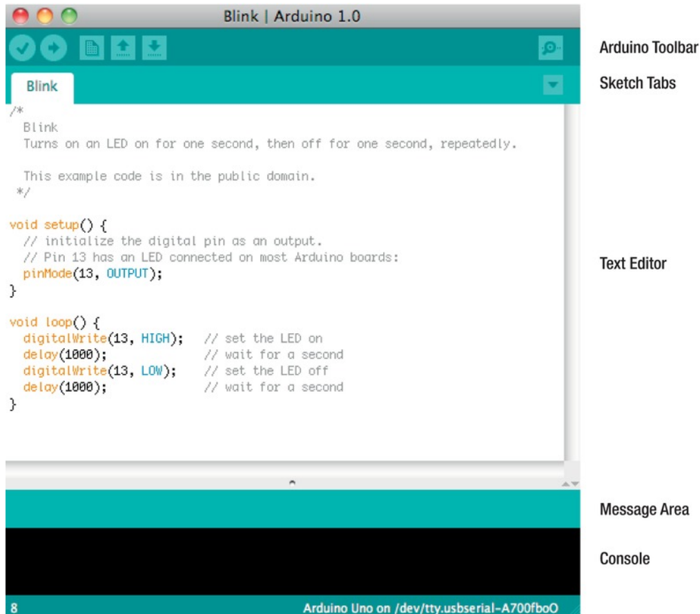
Figure 1-10. Arduino IDE
