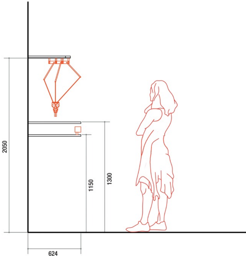
Figure 13-18. Robot setup
