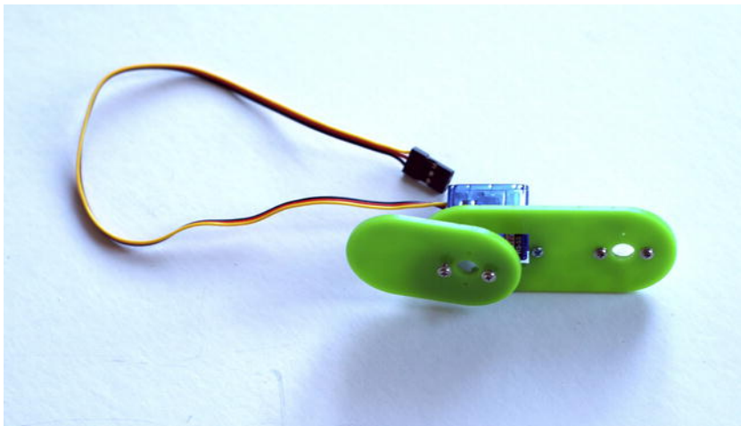
Figure 6-10. Arm assembled
