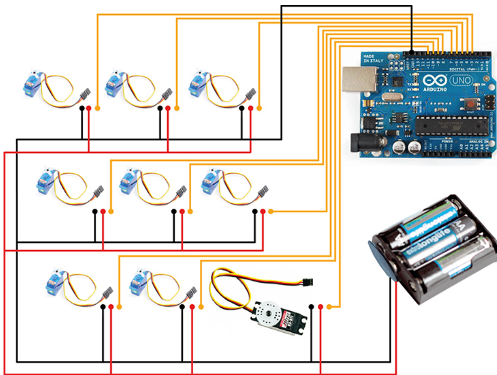
Figure 6-13. Circuit diagram
