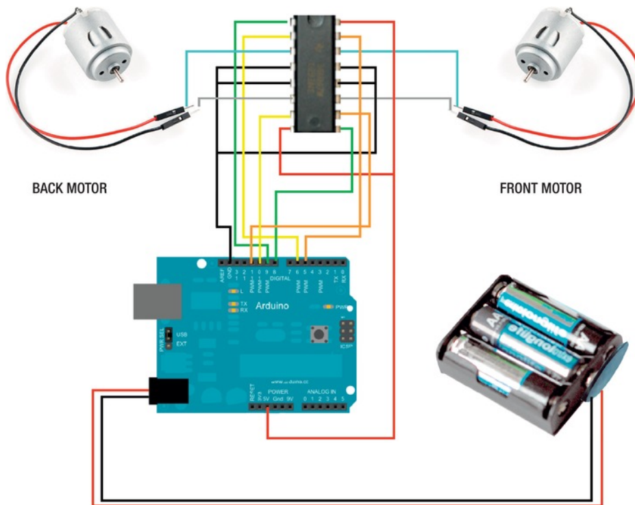
Figure 9-15. Circuit diagram
