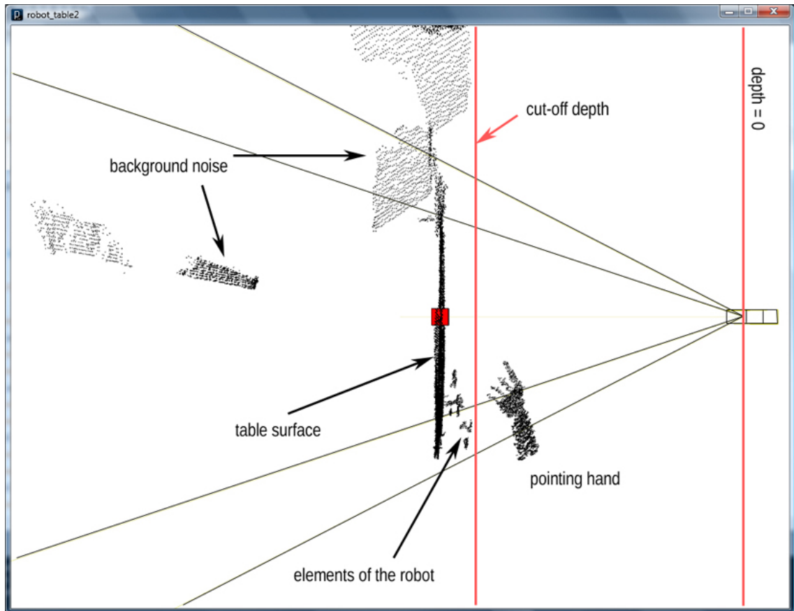
Figure 8-24. Point cloud filtering
