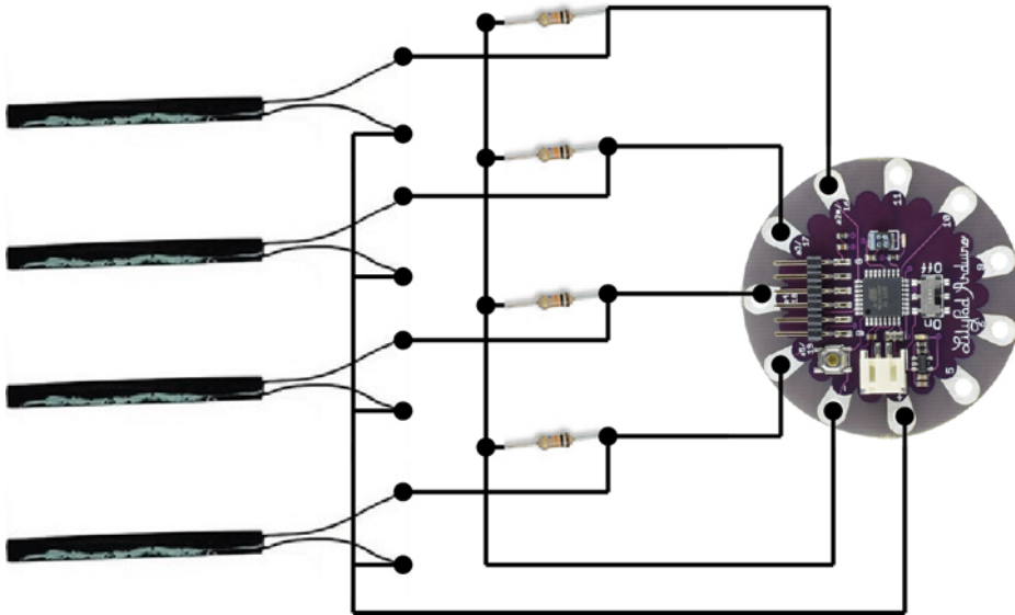
Figure 11-9. Flex sensors circuit
