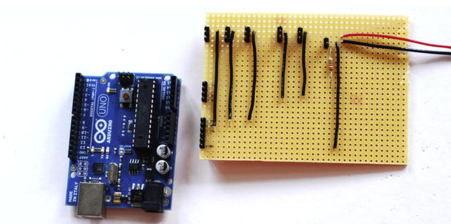
Figure 13-24. Finished board
