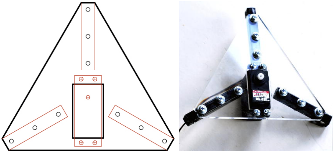
Figure 13-10. Effector drawing and assembly
