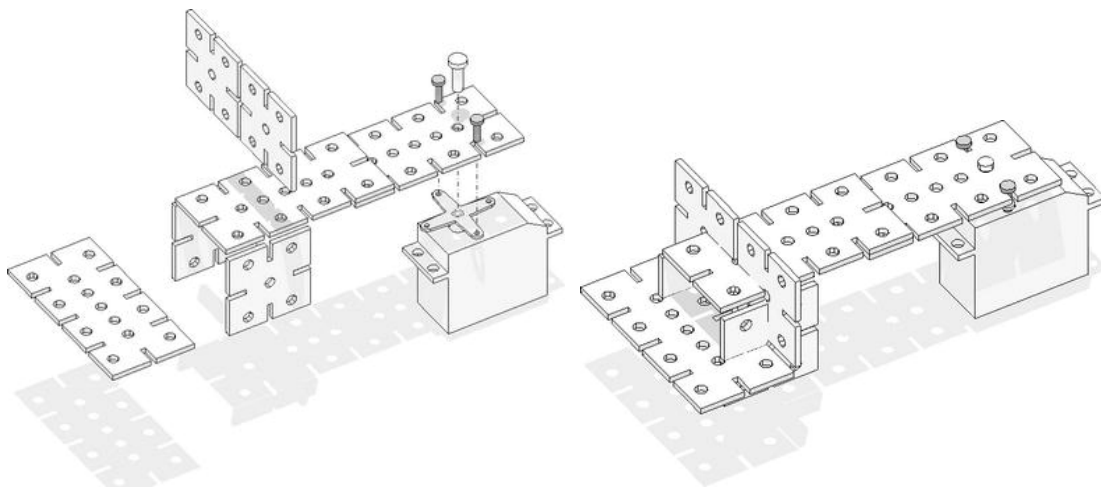
Figure 8-7. Part 2 assembly
