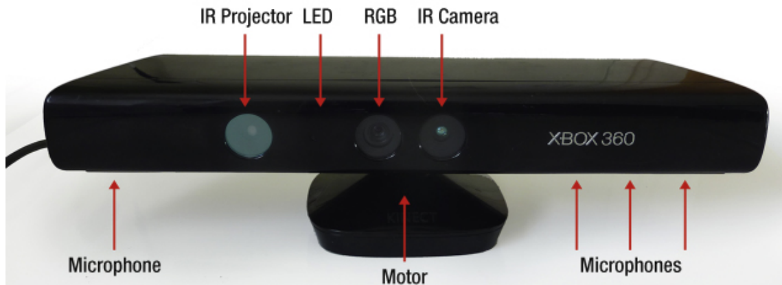
Figure 2-3. Kinect hardware
