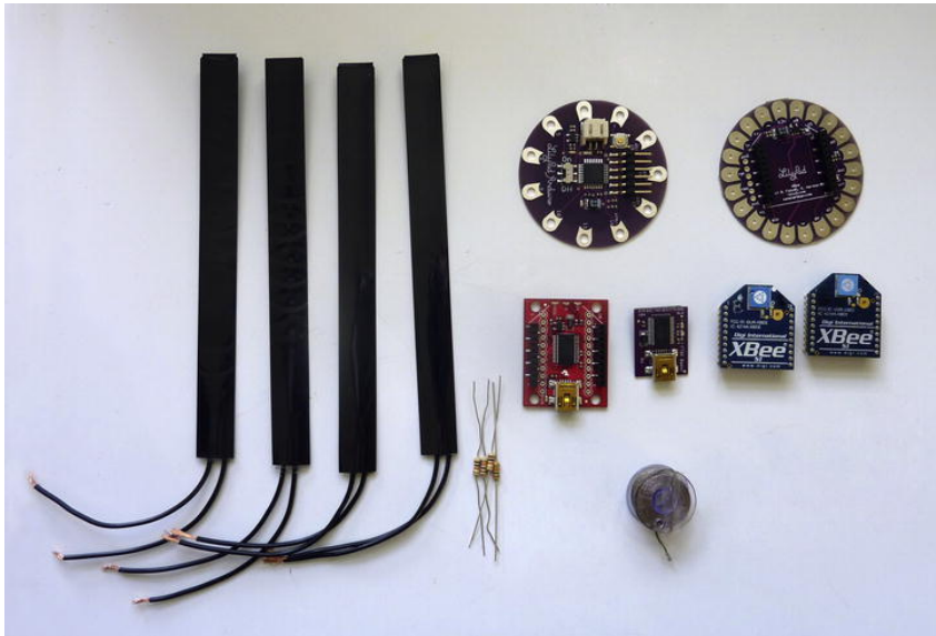
Figure 11-3. Project parts
