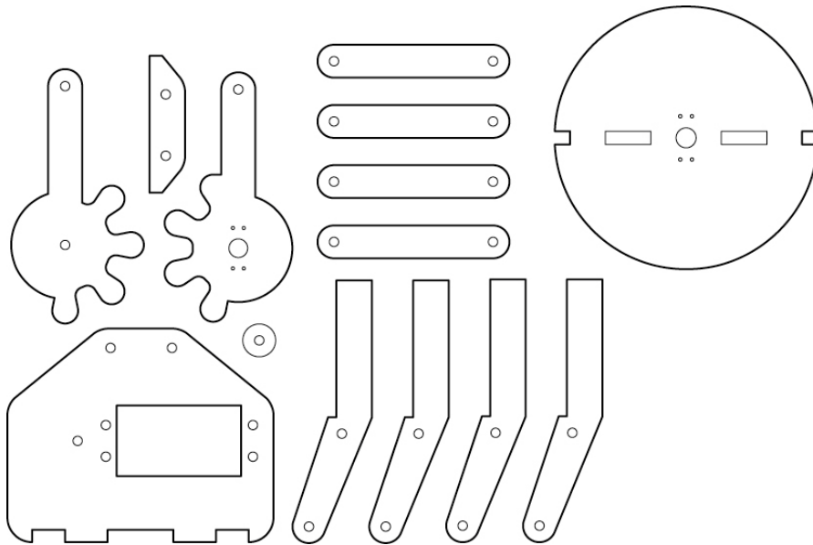
Figure 13-11. Gripper parts
