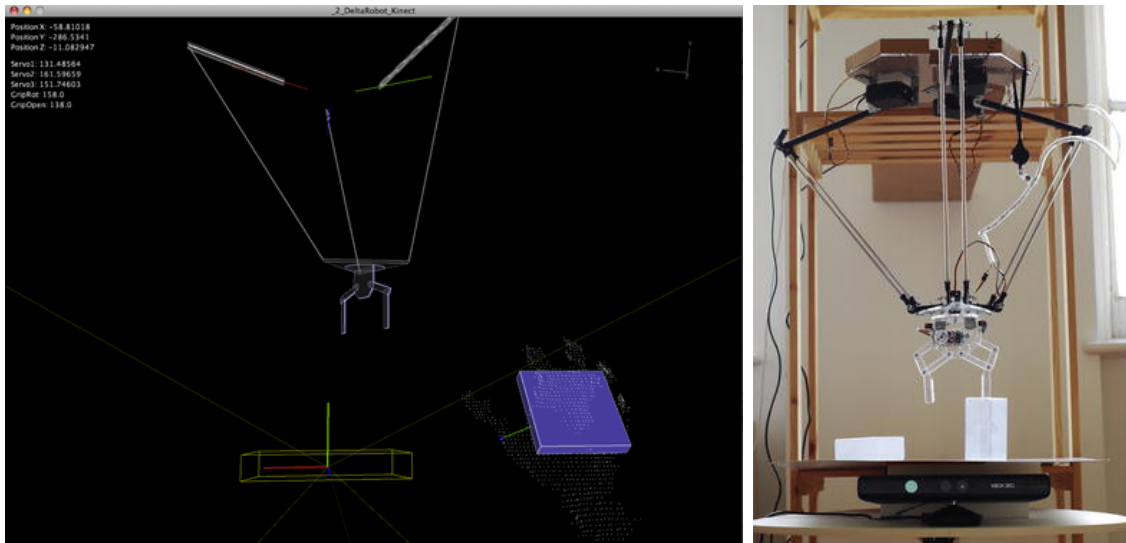
Figure 13-1. Delta robot simulation and physical robot
