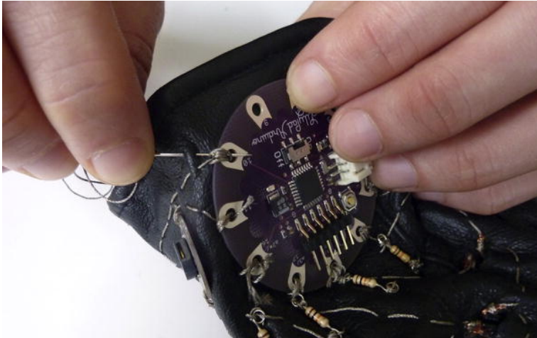
Figure 11-8. Sewing the circuit
