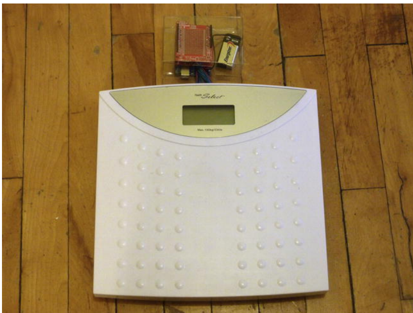
Figure 10-9. Scale finished and plugged to the Arduino and XBee module
