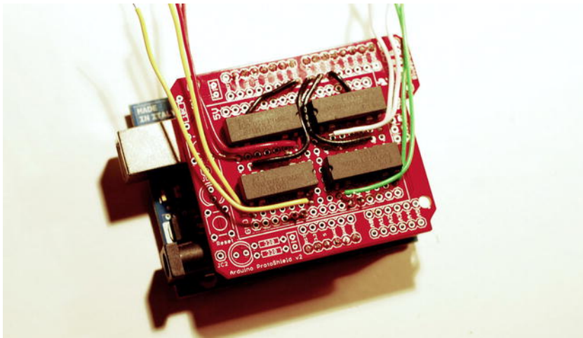
Figure 5-11. Finished shield
