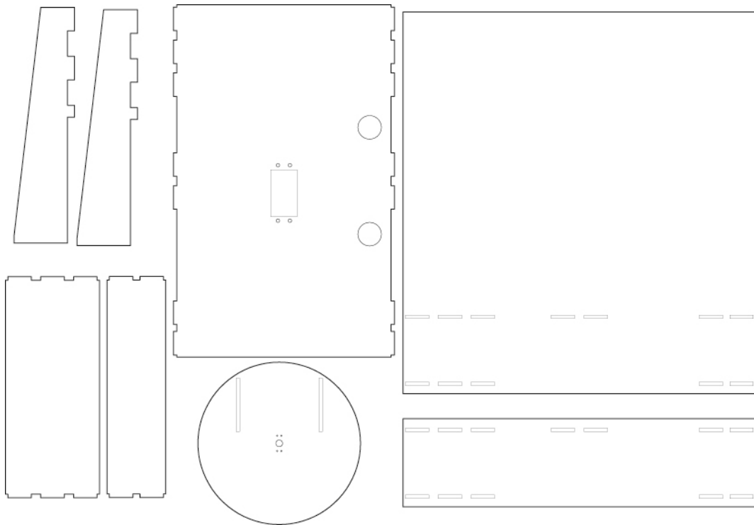
Figure 6-3. Stage parts
